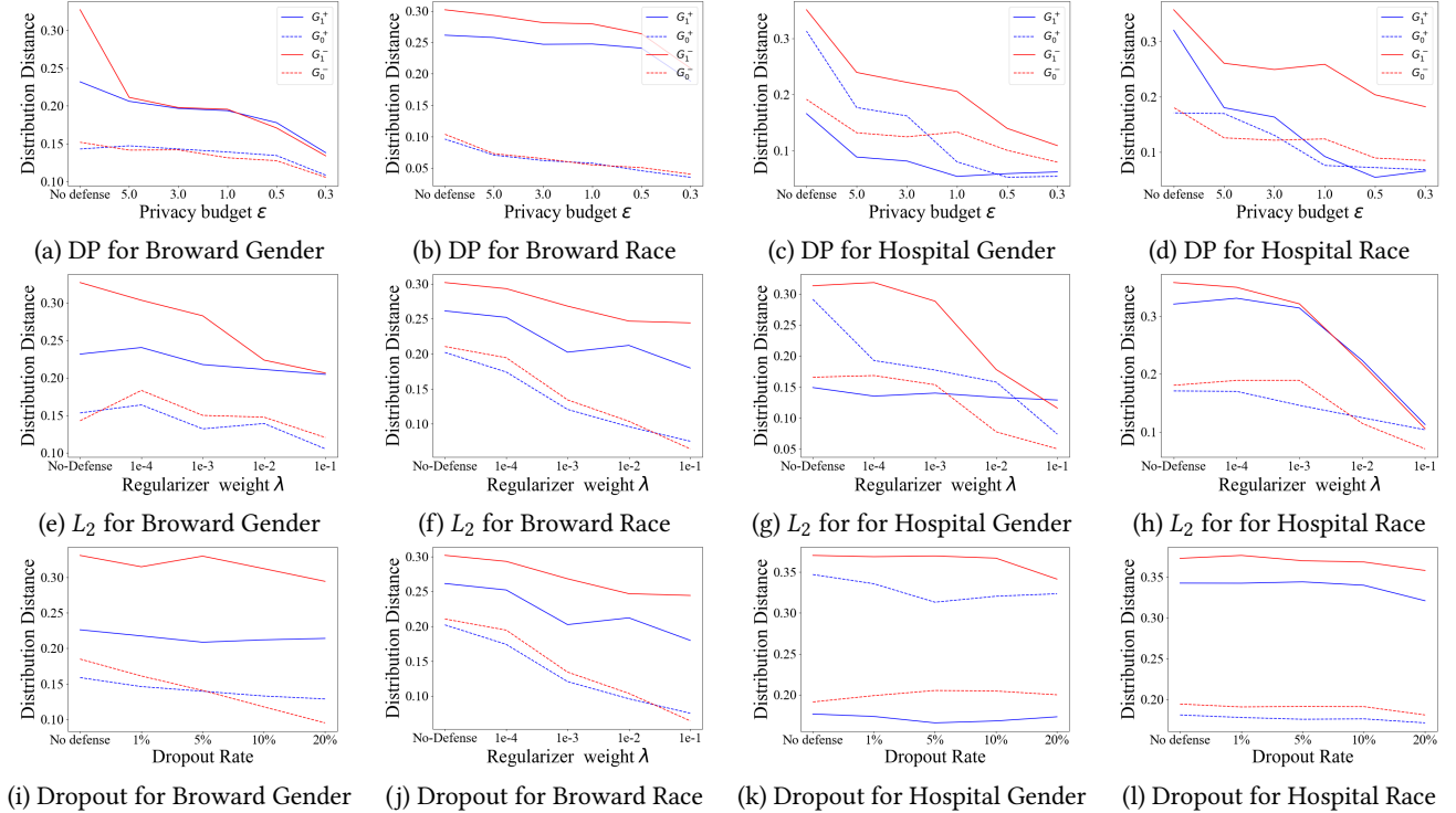
Figure 8: Change of CSV distribution distance each subgroup and the entire population with increase of defense strength.
